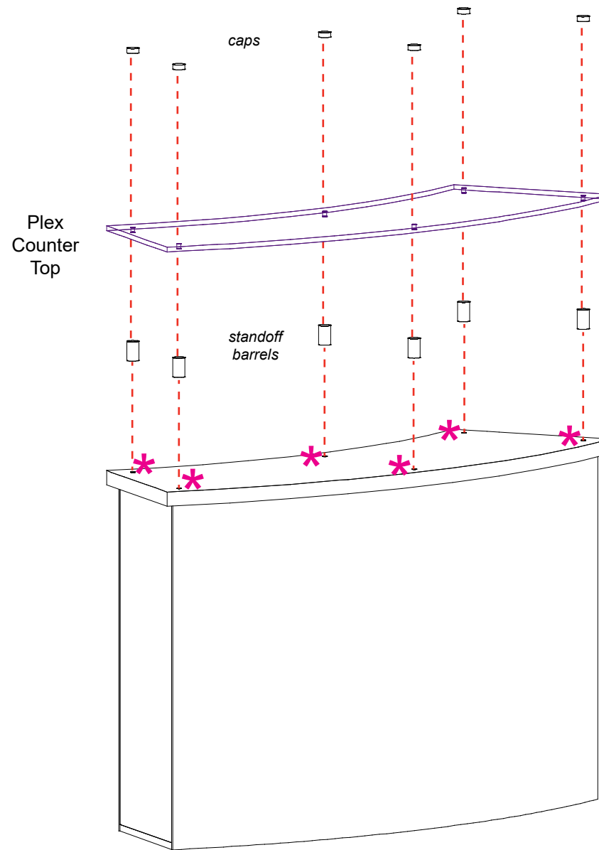
FRONT VIEW
